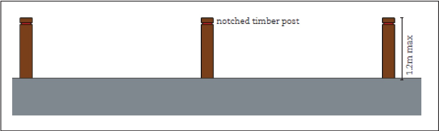
Figure 13 - Fencing Detail 3 - Public Open Space - Conservation
